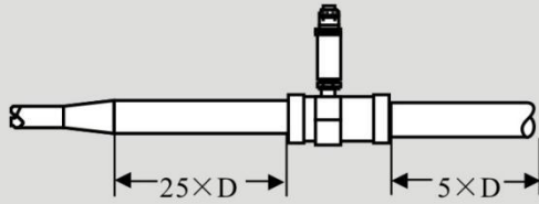
Concentric expander
