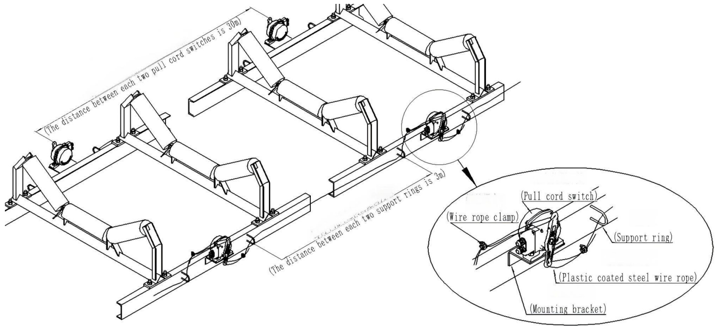
Installation diagram
