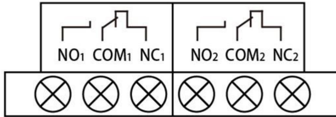
Pull cord switch wiring diagram)
