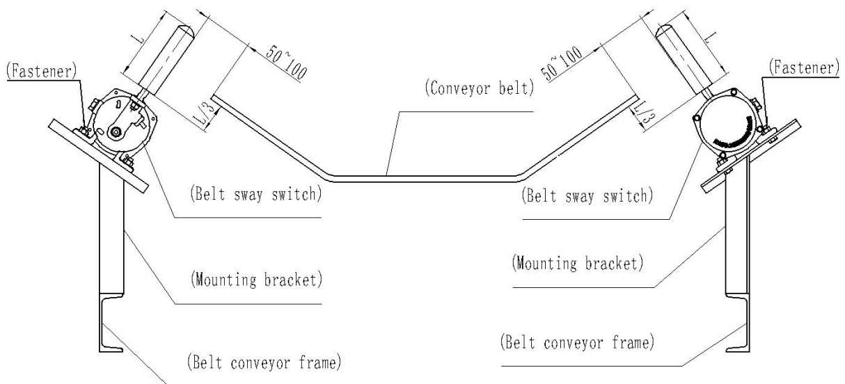
Installation indication diagram
