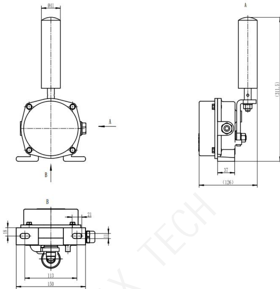
Appearance size chart ( Units: mm )
