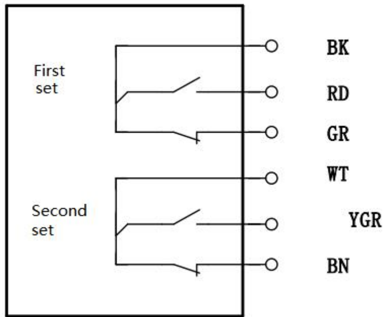
Belt sway switch wiring diagram
